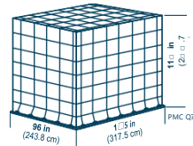
IATA ULD code: PMC Q7 Universal general-purpose flat pallet for lower holds and main decks. Tare weight: 120 kg (265 lb) Volume: H 299.7 cm (118 in), 21.2 m 3 (750 ft 3 )
