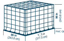
IATA ULD code: PMC Q6 Universal general-purpose flat pallet for lower holds and main decks. Tare weight: 120 kg (265 lb) Volume: H 243.8 cm (96 in), 17.0 m 3 (600 ft 3 )
