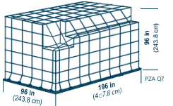
IATA ULD code: PZA Q7 Universal general-purpose flat pallet for lower holds and main decks.
