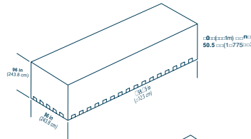
747F nose cargo door only
