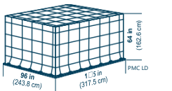
IATA ULD code: PMC LD Universal general-purpose flat pallet for lower holds and main decks. Tare weight: 120 kg (265 lb) Volume: H 162.6 cm (64 in), 11.5 m 3 (407 ft 3 )
