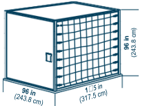
ULD code: AMA rectangular container on P6P base Main-deck container. Door is canvas with built-in net door straps. Maximum gross weight: 6,804 cm (15,000 lb) Tare weight: 350 kg (772 lb),
