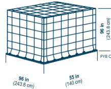
IATA ULD code: PYB Q6 Universal general-purpose flat pallet for lower holds and main decks.
