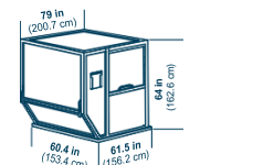
IATA ULD code: RKN contoured cool container Half-width lower hold insulated container with one angled end. Door is solid. Most examples are forkliftable. Door opening: 54 x 55-in (137 x 140-cm) Maximum gross weight: 1,588 cm (3,500 lb) Tare weight: 210 kg (463 lb)
