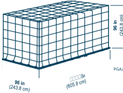
IATA ULD code: PGA/PGF Q6 Universal general-purpose flat pallet for lower holds and main decks.
