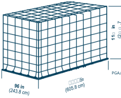
IATA ULD code: PGA/PGF Q7 Universal general-purpose flat pallet for lower holds and main decks.
