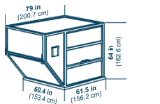
IATA ULD code: AKE contoured container Half-width lower hold container with one angled side. Door is either canvas or solid. Door opening: 58 x 61-in (147 x 155-cm) Maximum gross weight: 1,588 cm (3,500 lb) Tare weight: 82 kg (181 lb) AS1825 volume: 4.5 m 3 (159 ft 3 )
